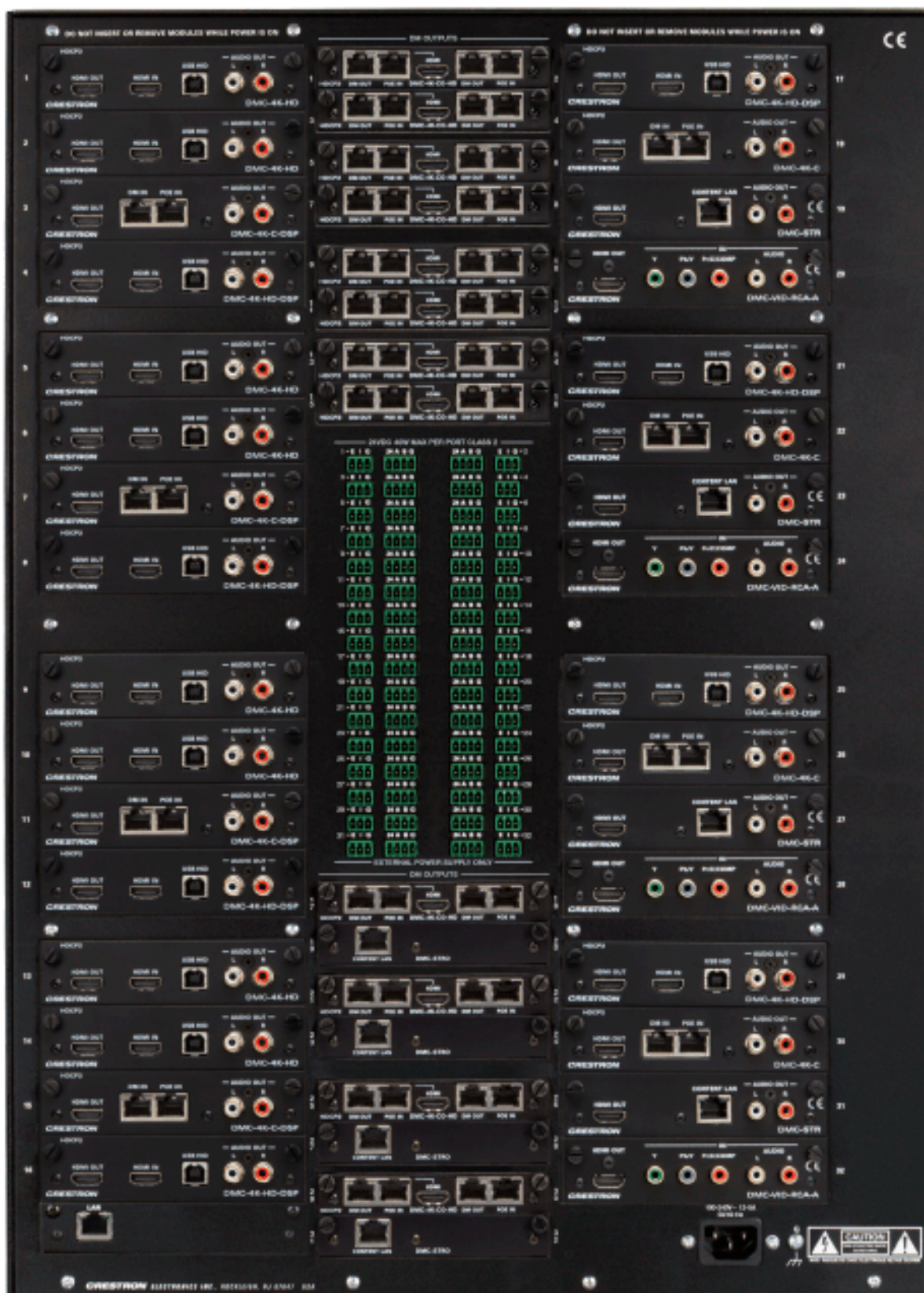
DM-MD32X32-RPS – Rear view with I/O cards installed
