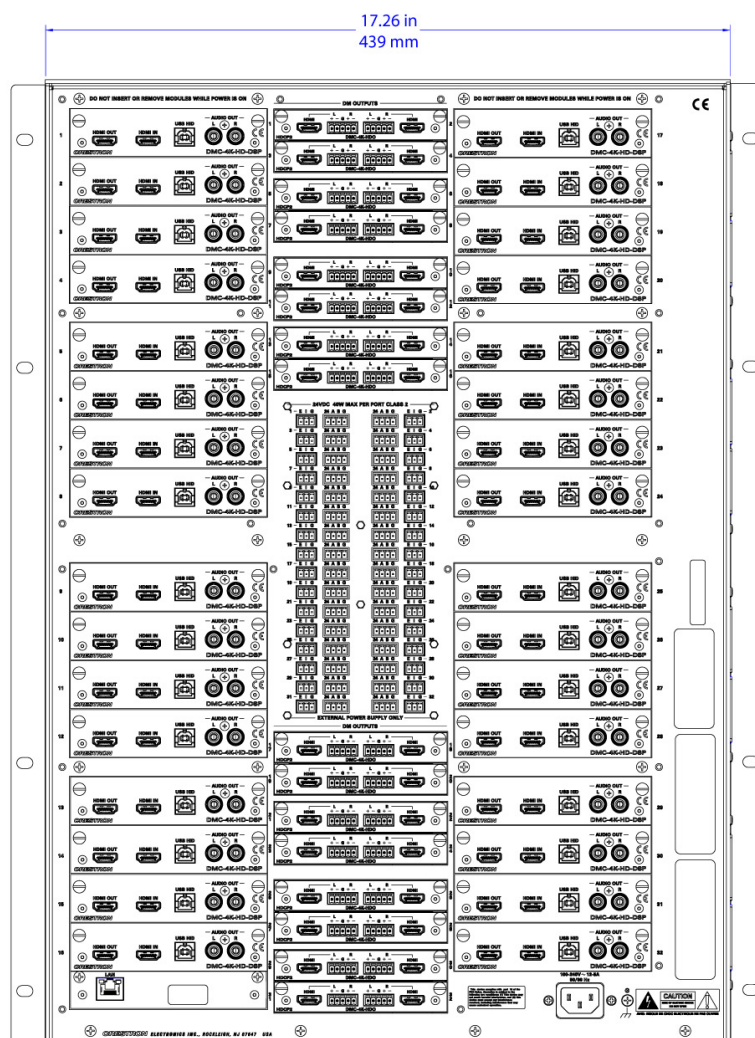
NOTE: Shown with input and output cards installed. All input and output cards sold separately.
